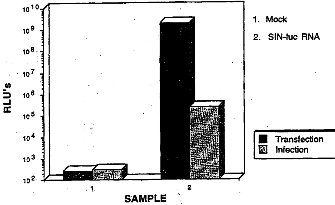
Figure 9: Sindbis-luciferase Vector Packaging in LTR/SindIBspE cells
